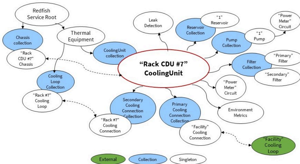
Figure 1: Resource Tree for Thermal Equipment
