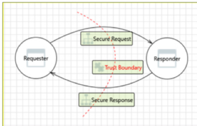
Figure 1 — SPDM threat model
